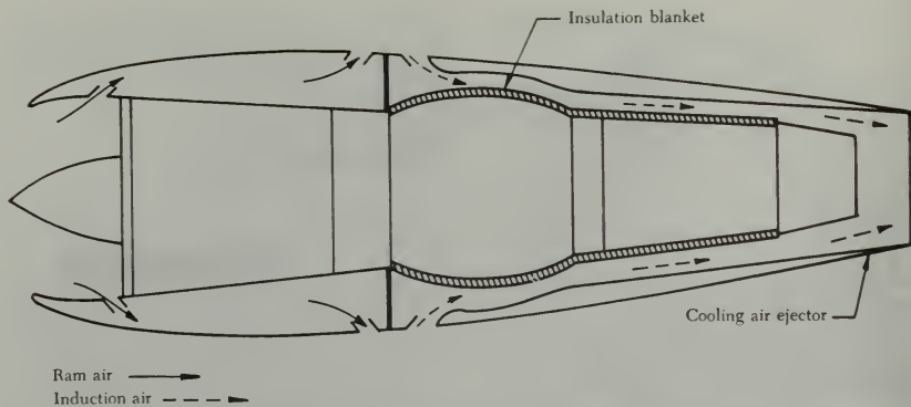
FIGURE 1-63. Exhaust system insulation blanket.
